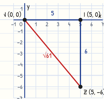
one possible triangle IZN
