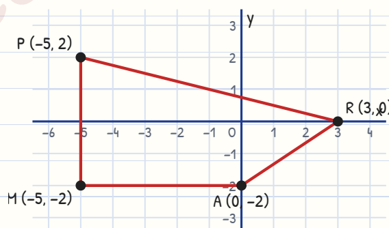
AM \parallel x-axis, MP \parallel y-axis, AM \perp MP
