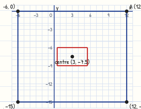
dining room 18\text{ ft} \times 15\text{ ft} and the 5\text{ ft} \times 3\text{ ft} table
