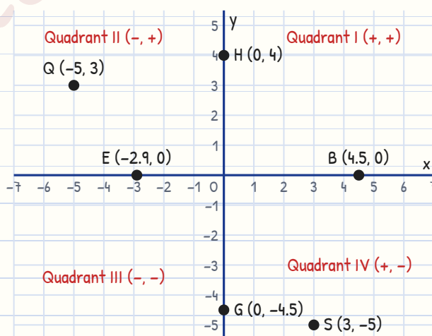
the four quadrants and points on the axes
